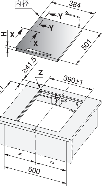
CookTop V4000 I402 (31144)
